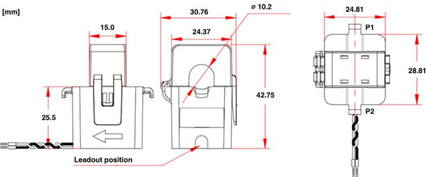
Product dimensions drawing
